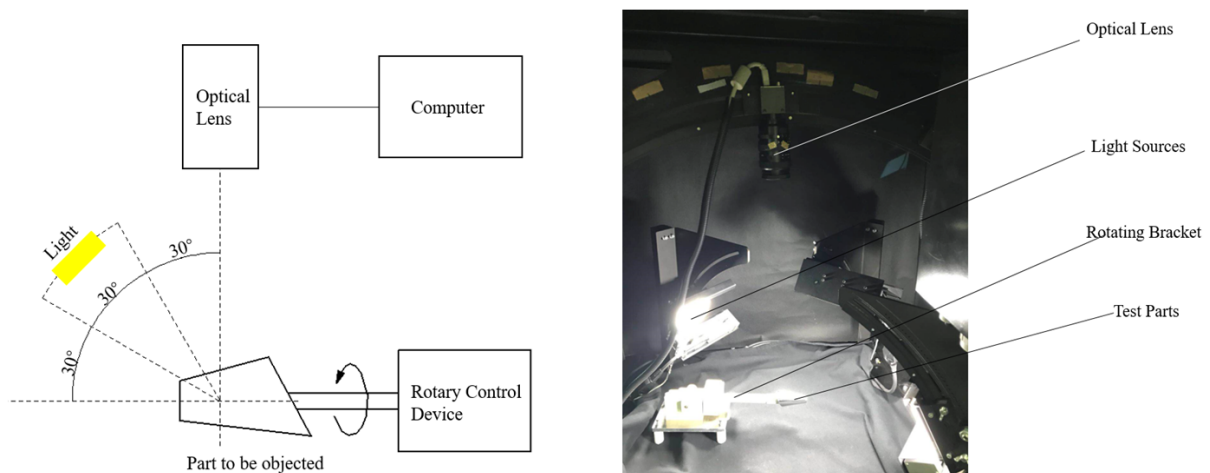
FIGURE 2. Light source and camera system schematic and physical map
