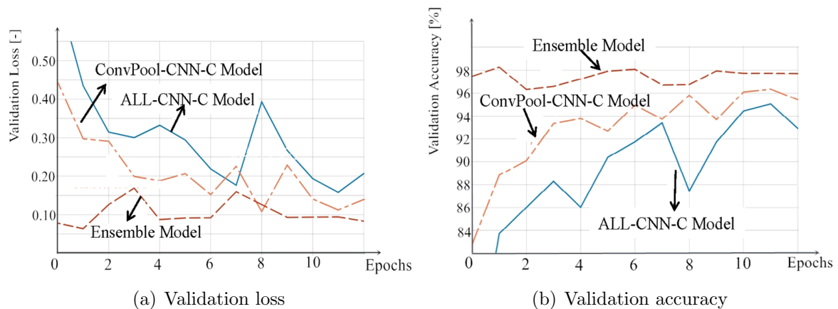
FIGURE 7. Validation loss and validation accuracy of 3 models
