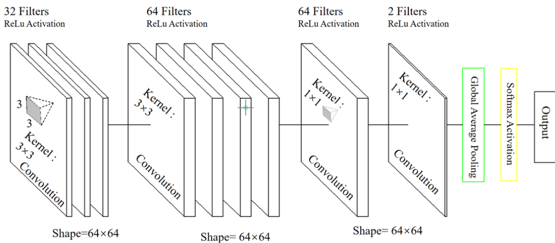
FIGURE 5. ALL-CNN-C based model
