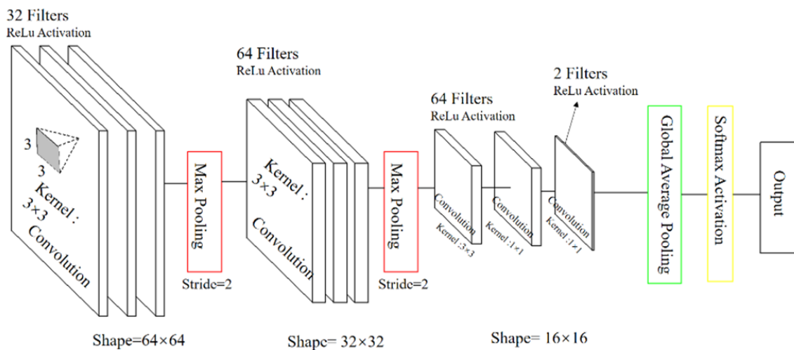
FIGURE 4. ConvPool-CNN-C based model
